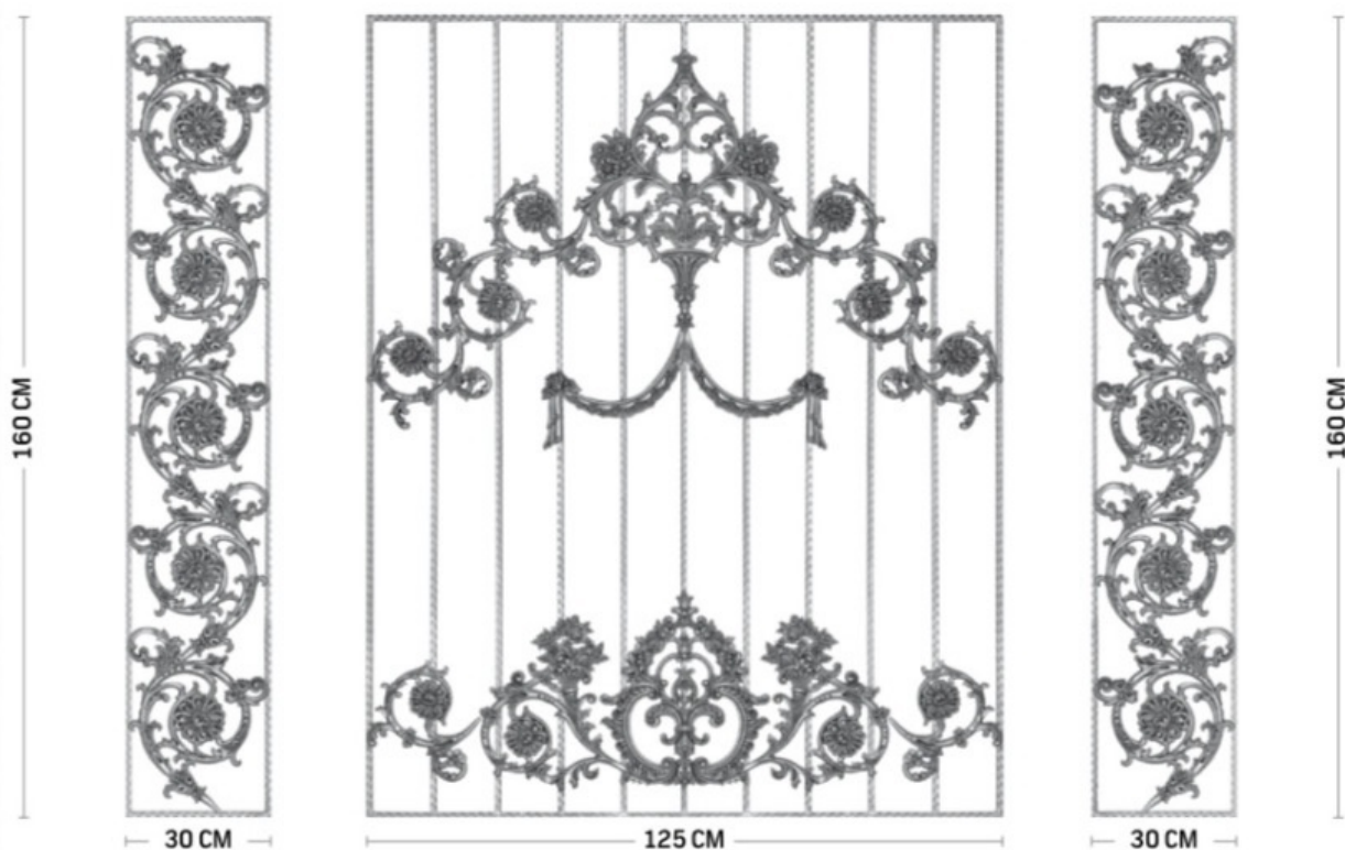
1464 Weight:13.66 KG
