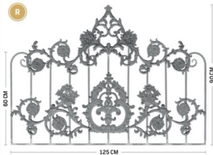
1469 Weight: 22.4 KG
